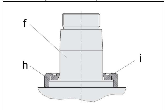
Figure 8: Metallic wiper
