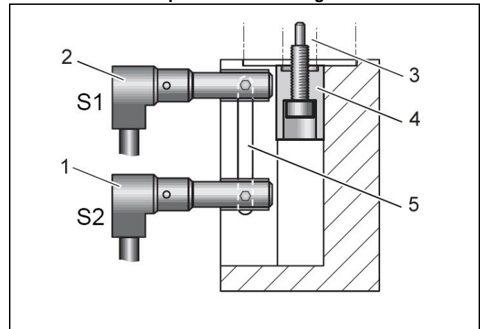
Figure 11: Design of the electrical position monitoring
