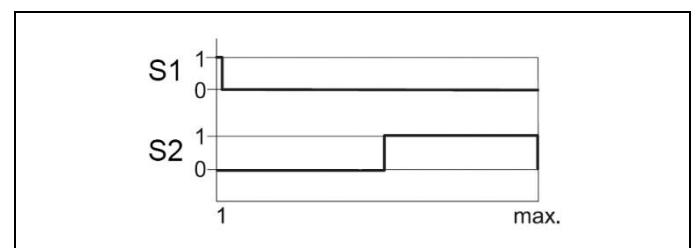
Figure 12: Signal course - clamping
